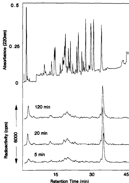
FIGURE 2: Analysis of tryptic digests of ornithine aminotransferase after rapid inactivation by aminohexynoate and delayed reduction. Inactivations were conducted by use of 10 mM [ ^{14}\text{C} ]aminohexynoate. Sodium borohydride (1 mg/mL) was added at the intervals indicated. Denaturation and tryptic digestion were as described in the text. Chromatographic conditions: flow rate, 1.5 mL/min; solvent A, 0.1% TFA in water; solvent B, 0.1% TFA in 70% acetonitrile in water. For elution, after 2 min at 0% solvent B, a gradient from 0% to 50% solvent B was developed in 30 min, followed by 6 min at 50% and a gradient over 2 min to 95% solvent B; the column was then washed for 5 min at 95% solvent B.
