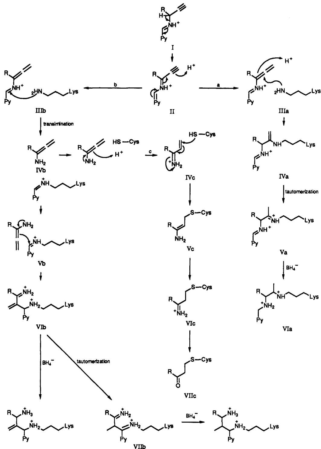
Scheme I: Proposed Mechanisms for the Reaction of Ornithine Aminotransferase with Aminohexynoate
