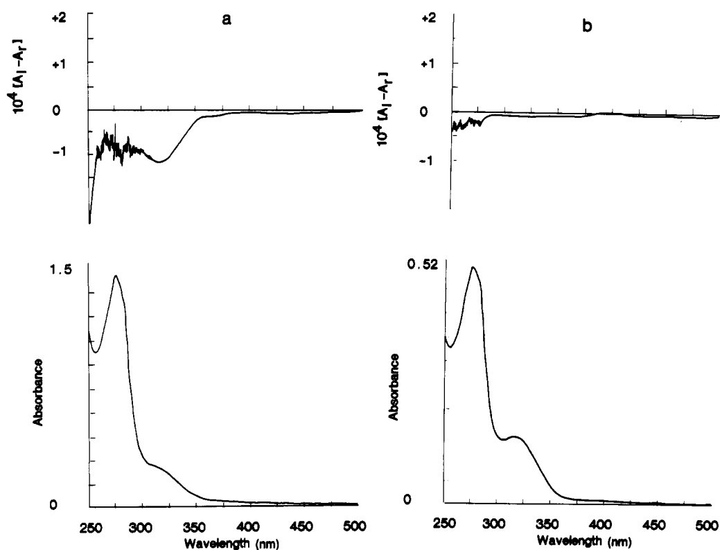
FIGURE 4: Absorbance and CD spectra of 320 nm absorbing peptides. (a) Labeled peptide (TR4) obtained after inactivation of ornithine aminotransferase (20 mg) with aminohexyanoate and reduction with borohydride. (b) Pyridoxyl-peptide arising from borohydride reduction of ornithine aminotransferase (10 mg) that had not been treated with aminohexyanoate.
