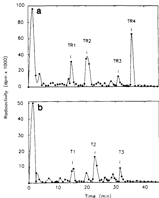
FIGURE 1: Distribution of radioactivity in preparative separations of tryptic digests. Tryptic digests of denatured ornithine aminotransferase, inactivated by use of 1.3 mM [ ^{14}\text{C} ]aminohexynoate, were separated by reversed-phase HPLC as described in the text and using the gradient described in Figure 3. Column eluate was monitored at 220 and 325 nm. The pattern of radioactivity in the case of the sample from the reduced enzyme (a) was obtained from chromatography of all 2.5 mg of the sample whereas in the case of the digest from the unreduced sample (b) the radioactivity pattern is from a portion (0.8 mg).
